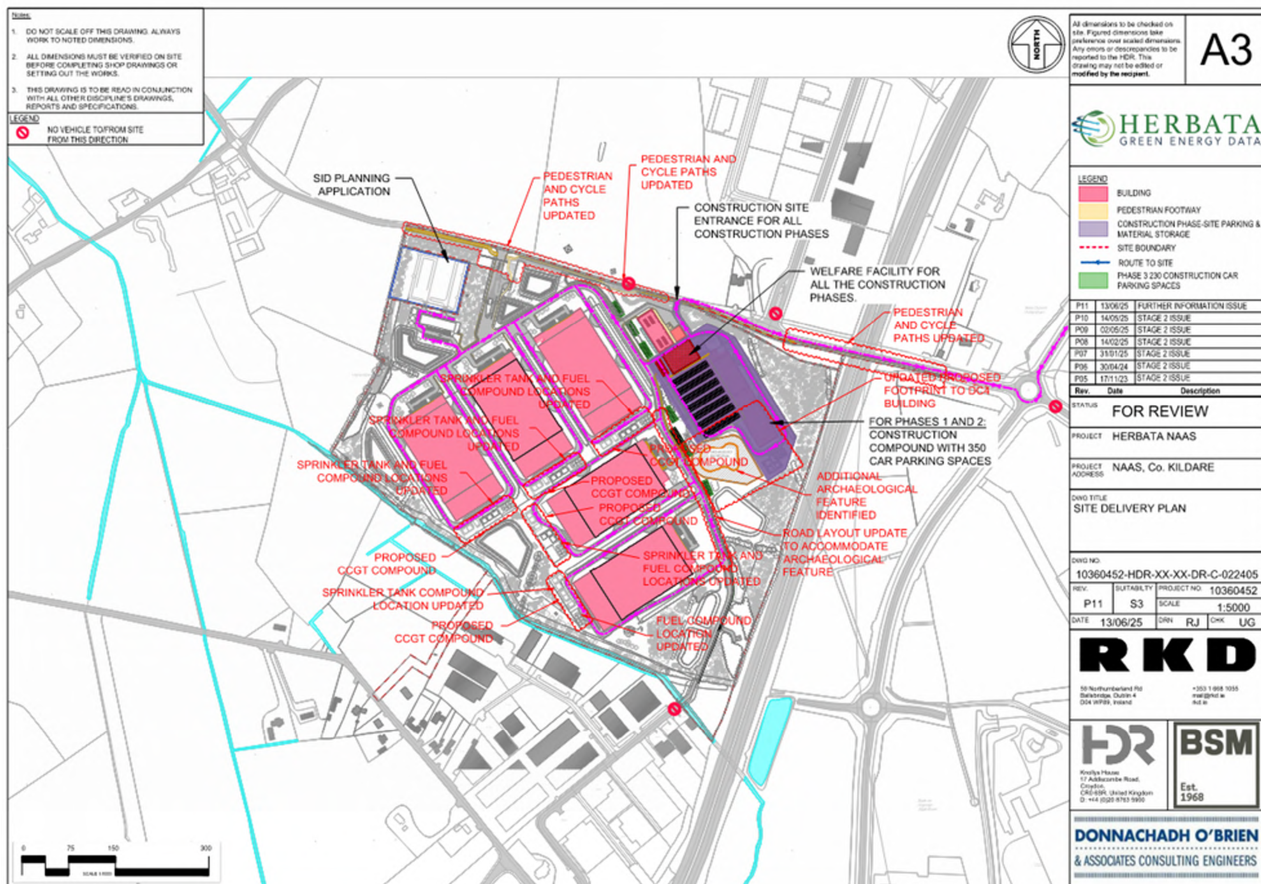
Figure 4-3. Site delivery plan 1:5,000
