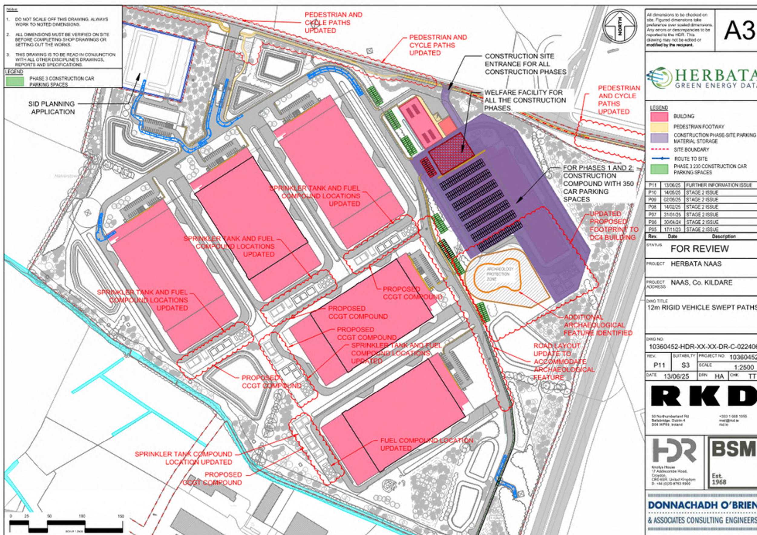
Figure 4-4. 12m Rigid vehicle swept paths 1:2,500.
